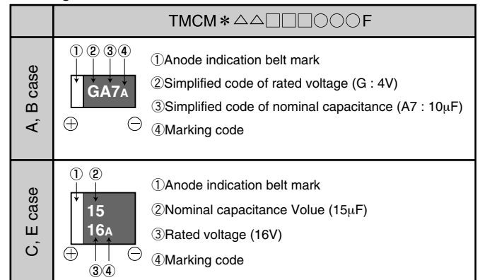
Marking indication TCMC series
