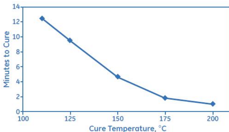
Figure 1: Addisil 6101 Silicone Adhesive Cure Time vs Temperature
